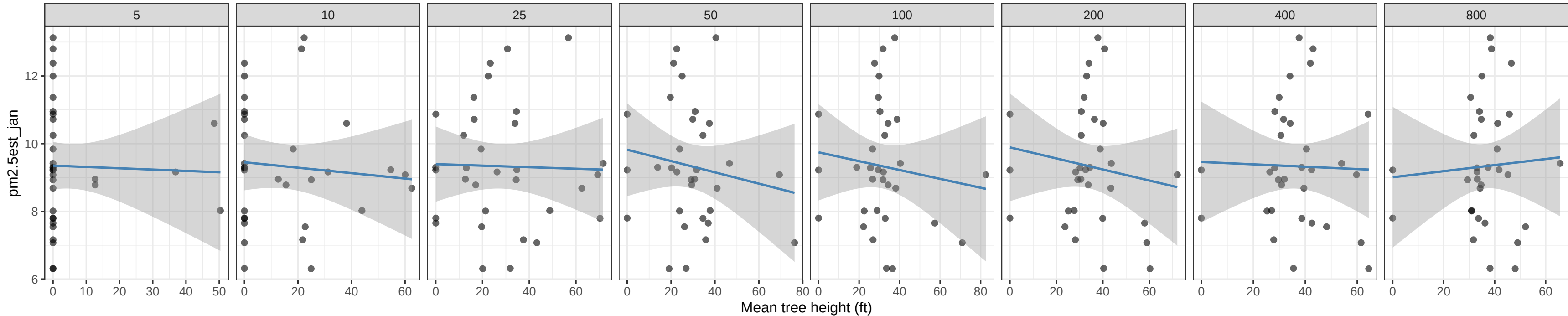
pm2.5est_jan vs Mean tree height (ft) by buffer radius
